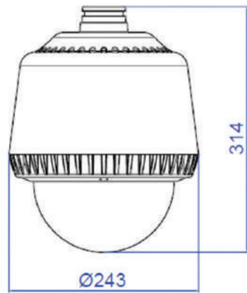
FW8706-HNP 2MP IR Speed Dome
