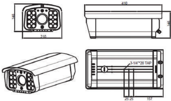
▲ FW9305-GSM 2MP Global Shutter ANPR/LPR
